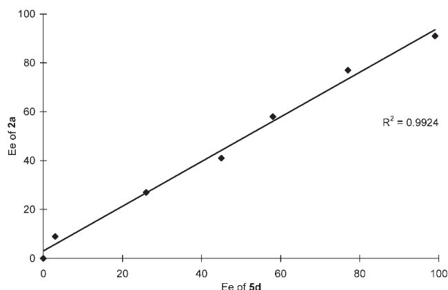
Figure 3. Linear effect in the 5d -catalyzed reduction of ketimine 1a with trichlorosilane.
